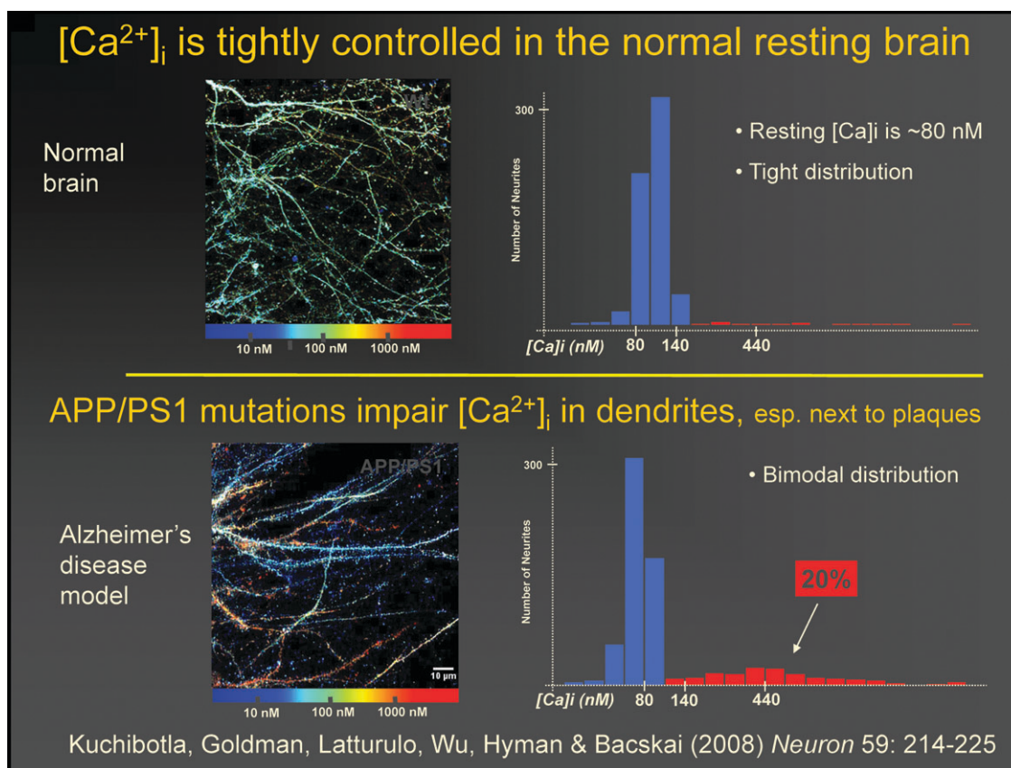
Fig. 14 Two-photon imaging of yellow cameleon 3.60 79 in brains of transgenic mice, without or with APP1/presenilin mutations to generate plaques modeling Alzheimer's disease. Low to high cytosolic [Ca 2+ ] i level are shown in blue to red pseudocolors respectively. In the disease model, 20% of neurons show a distinctly higher cytosolic [Ca 2+ ] i , especially in the vicinity of disease plaques. Figure donated by Dr Brian Bacskai and related to Kuchibotla et al. 60
