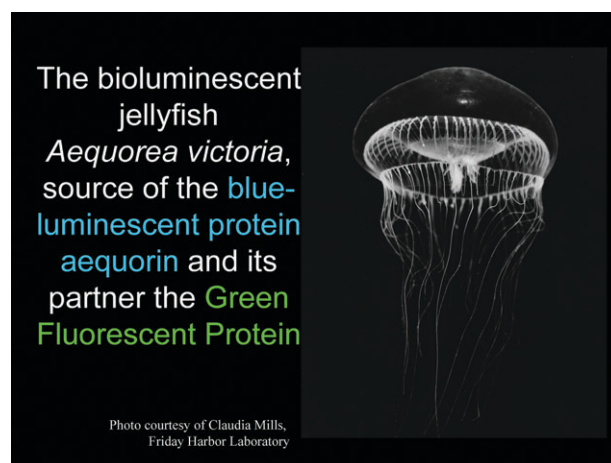
Fig. 2 The jellyfish Aequorea victoria or Aequorea aequorea from which aequorin and Green Fluorescent Protein were isolated. Photo courtesy of Dr Claudia E. Mills, Friday Harbor Laboratories.
