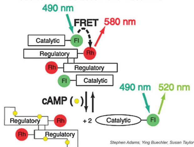
Fig. 1 Schematic cartoon showing how cAMP-induced dissociation of regulatory from catalytic subunits of protein kinase A (PKA) can be reported by loss of FRET from fluorescein to rhodamine labels.
