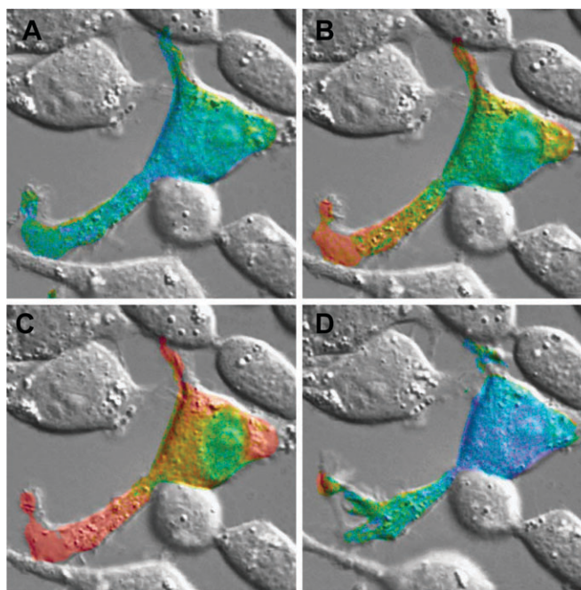
Fig. 10 A fibroblast transfected with a reporter 47 for the tyrosine kinase activity of the receptor for epidermal growth factor (EGF). The extent of FRET, indicating the extent of phosphorylation of the reporter, is shown in pseudocolors ranging from blue (negligible phosphorylation) to red (maximal phosphorylation). These colors are superimposed on differential interference contrast images to show cellular morphology. The colored cell was the only one transfected within this field of view. At rest the indicator showed negligible phosphorylation (A), but upon stimulation with EGF, phosphorylation (shown by warmer pseudocolors) started at the periphery of the cell (B) and spread towards the nucleus (C). After EGF was removed, the tide of phosphorylation receded back towards the most peripheral tip at the far left end of the cell (D).
