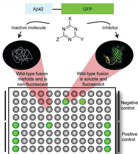
Fig. 15 High-throughput screening of combinatorial drugs to find inhibitors of aggregation of Aβ, the Alzheimer's disease peptide. Inhibition of aggregation allows an Aβ42–GFP fusion to become fluorescent. Reprinted with permission from Fig. 1 of Kim et al. 61
