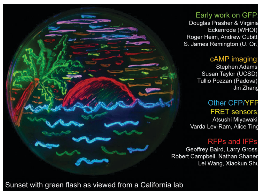
Fig. 21 Key collaborators for the work described in this lecture, and a glowing California sunset in a Petri dish, drawn with multiple colors of bacteria expressing fluorescent proteins.
