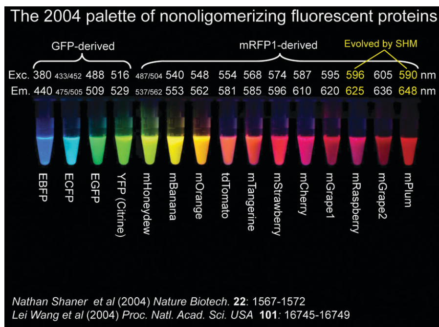
Fig. 12 Monomeric or tandem dimeric fluorescent proteins derived from Aequorea GFP or Discosoma RFP, expressed in bacteria and purified. This photo is a time exposure of fluorescences excited at different wavelengths and viewed through different cutoff filters.
