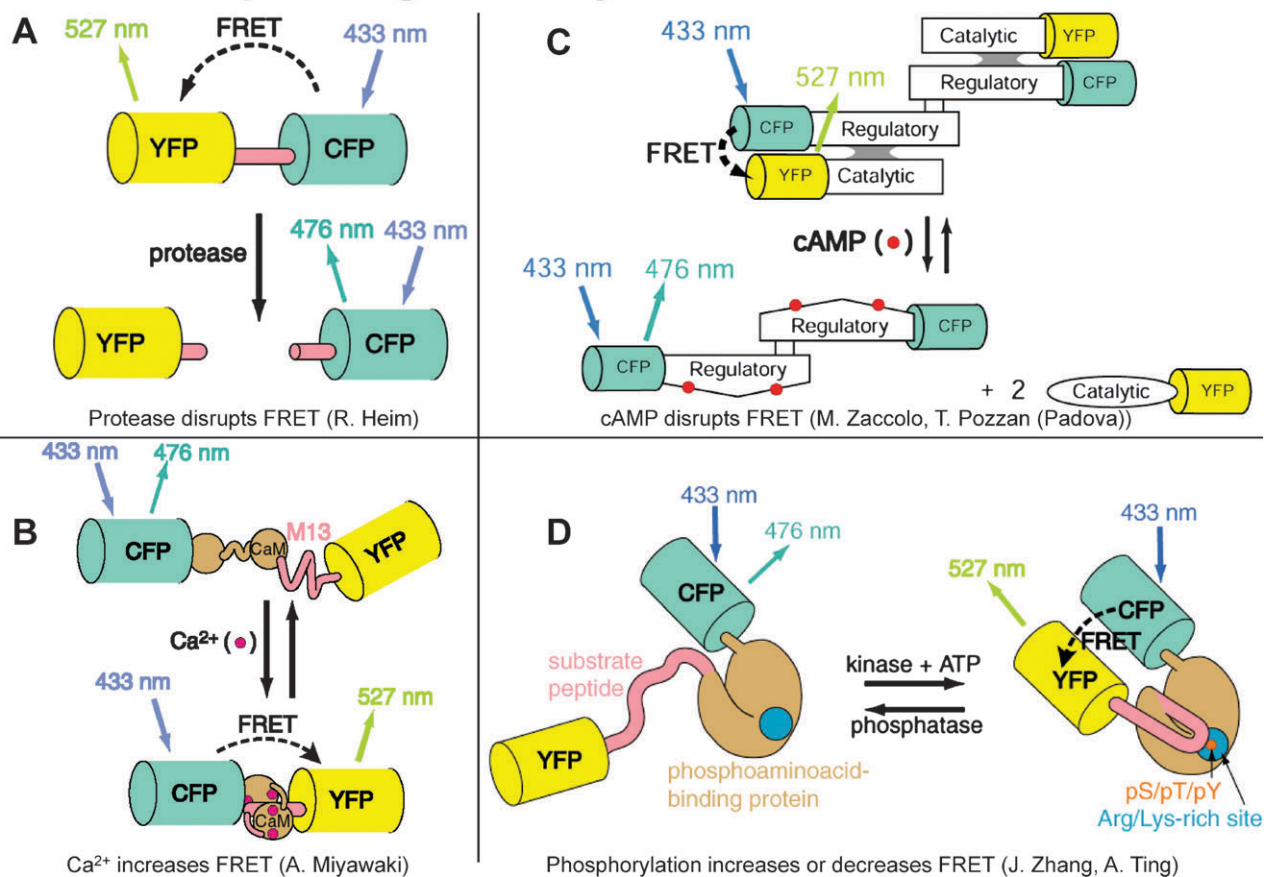
Fig. 7 Schematic cartoons of genetically encoded fluorescent indicators based on FRET from CFP to YFP, to report (A) protease activity, (B) \text{Ca}^{2+} concentrations, (C) cAMP concentrations, and (D) the balance between protein kinase and phosphatase activity.
