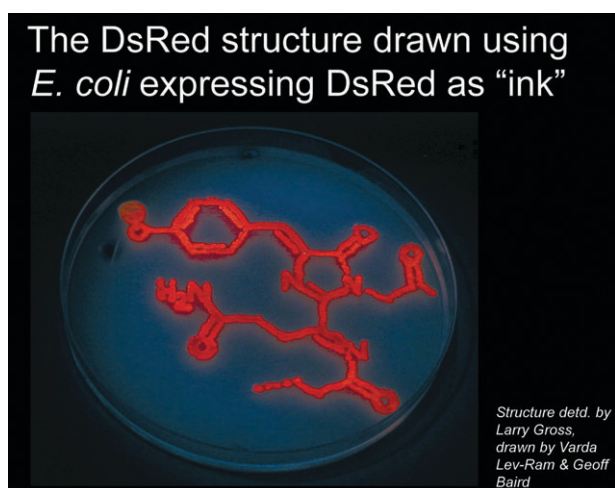
Fig. 11 Chromophore structure 52 of DsRed, drawn on a Petri dish using bacteria expressing the protein and showing its beautiful red fluorescence.
