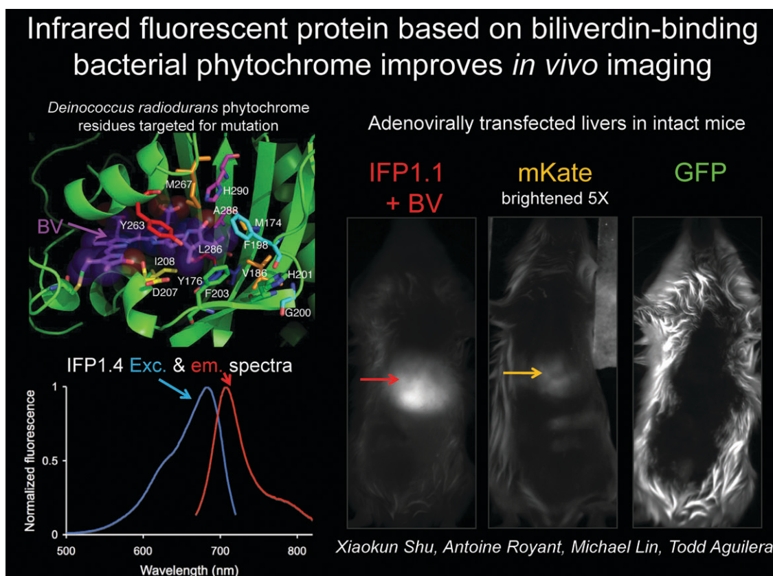
Fig. 19 An infrared-fluorescing protein (IFP) can be evolved from a phytochrome from Deinococcus radiodurans . Upper left: crystal structure of the wild-type phytochrome (PDB: 1ztu) 81 with its chromophore, biliverdin, in purple, and residues targeted for mutagenesis labeled. Lower left: Normalized excitation (blue) and emission (red) spectra of IFP1.4. Right: Liver fluorescence of intact living mice injected with adenoviruses encoding IFP1.1, mKate (an RFP previously advocated for in vivo imaging 82 ), or an enhanced GFP. Biliverdin (250 nmol) was injected intravenously 1 h before obtaining the IFP image. The mKate image was 5-fold brightened in software to render it visible. Belly fur was removed with depilatory cream but the skin was left unbroken. Arrows point to the liver. Note that the GFP images are dominated by autofluorescence, rendering the livers invisible. The much greater visibility in the highly pigmented liver of IFP compared to previous FPs demonstrates the value of very long excitation and emission wavelengths for in vivo fluorescence imaging.
