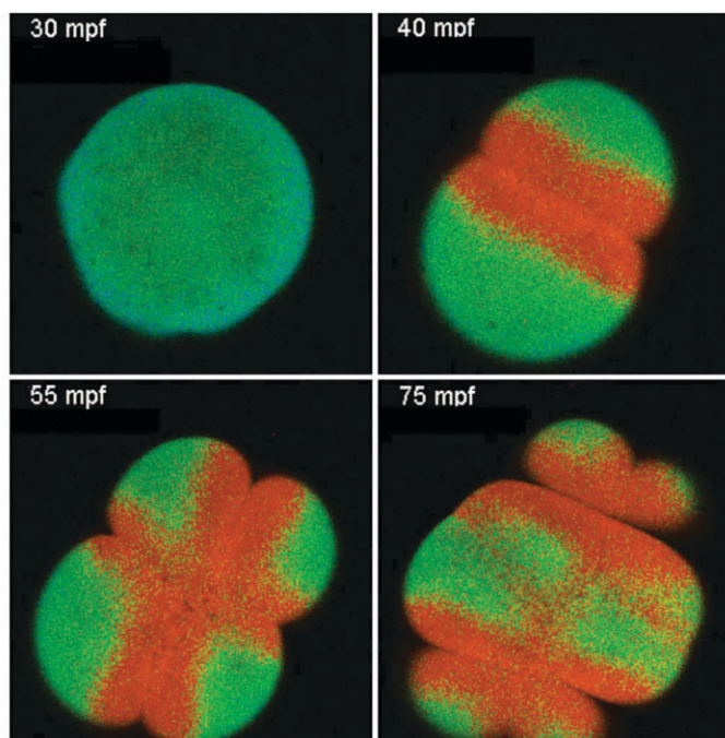
Fig. 9 Transgenic zebrafish embryo expressing yellow cameleon 2.60. 79 Single confocal z-plane, imaged every 5 s ('mpf' = minutes post fertilization). Images selected from a video kindly provided by Hide Mizuno & Atsushi Miyawaki, RIKEN, Japan.
