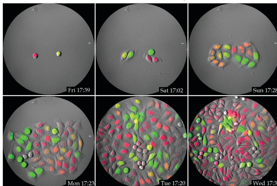
Fig. 16 Frames chosen from a time-lapse video of HEK293 cells growing and dividing in tissue culture while transfected with a two-color reporter of cell cycle progression. Green-fluorescing cells are actively undergoing mitosis, whereas red-fluorescing cells are in interphase. 62 Video courtesy of Asako Sawano & Atsushi Miyawaki, RIKEN.
