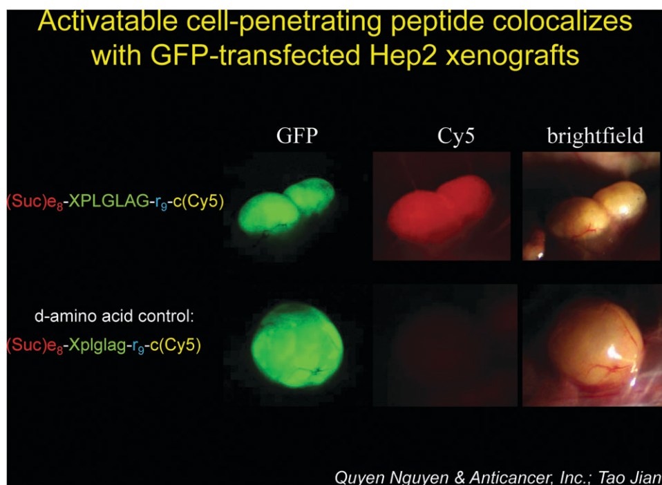
Fig. 20 Activatable cell penetrating peptides (ACPPs) localize to tumors in vivo . Hep2 (human laryngeal carcinoma) tumor cells stably transfected with EGFP were xenografted into nude mice. 3 weeks after implanting 5 \times 10^6 cells subcutaneously, the tumor had reached \sim 5 mm diameter. Top images: 6 h after systemic injection of an ACPP, 10 nmol succinyl-e 8 -XPLGLAG-r 9 -c(Cy5), the skin was removed over the tumor, and GFP fluorescence, Cy5 fluorescence, and reflected light images were acquired from the anesthetized animal. X denotes 6-amino hexanoyl, upper case letters represent L-amino acids, lower case letters are D-amino acids. PLGLAG is a sequence cleavable by matrix metalloproteinases-2 and -9. 74 Bottom panel: an analogous experiment with a matching negative control, succinyl-e 8 -Xplglag-r 9 -c(Cy5), in which the protease cleavage site has been changed to D-amino acids, rendering it protease-resistant. The lack of Cy5 signal in the tumor indicates that retention depends on cleavage by proteases.
