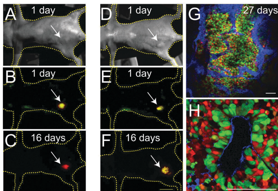
Fig. 17 Reporter of cell-cycle progression applied to benign (NMuMG) and malignant (HeLa) tumor implants in vivo . Fig. 3A–H from Sakaue-Sawano et al. , 62 reprinted with permission.
